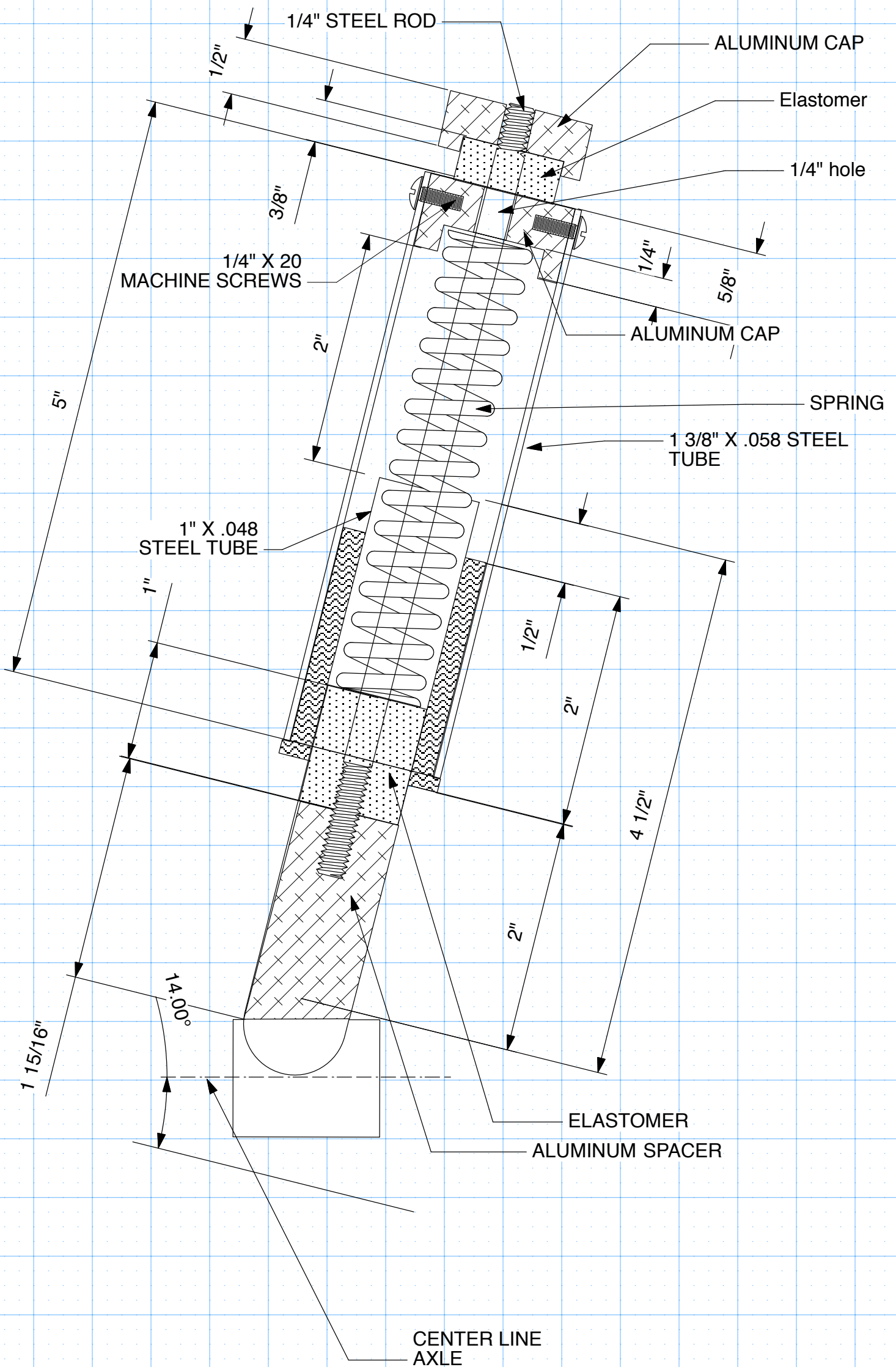
FRONT SHOCK DETAIL
