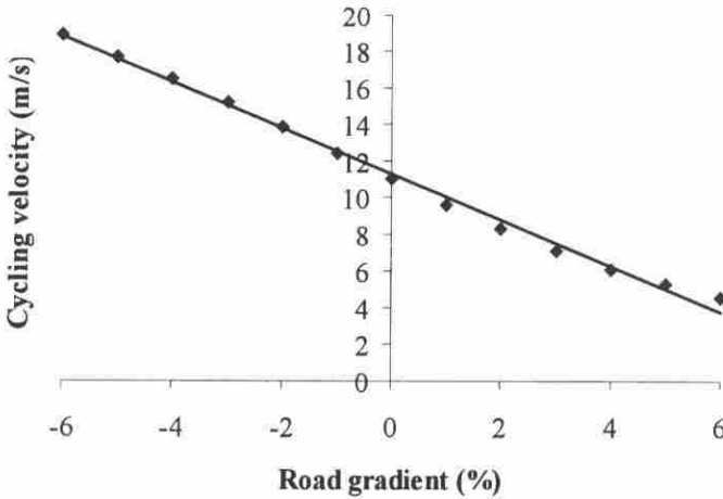
Figure 4 — The effects of road gradient on cycling velocity. Within the range of road gradients evaluated (–6 to 6%), the effects on cycling velocity were very nearly linear (cycling velocity [m/s] = 11.26 – 1.25 road gradient [%], R^2 > .99 ).
